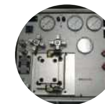
Servo Valve Analyzer (Moog F087-127)
